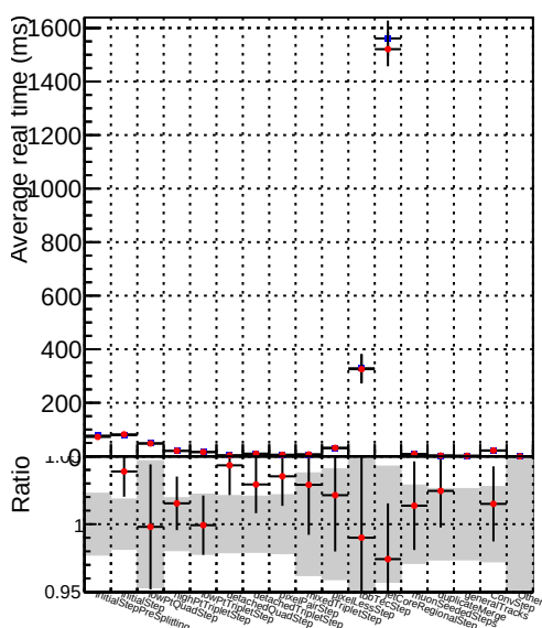
DQM_V0001_R000000001_Global_mkFit_baseline DQM_V0001_R000000001_Global_mkFit_BASELINE-2
