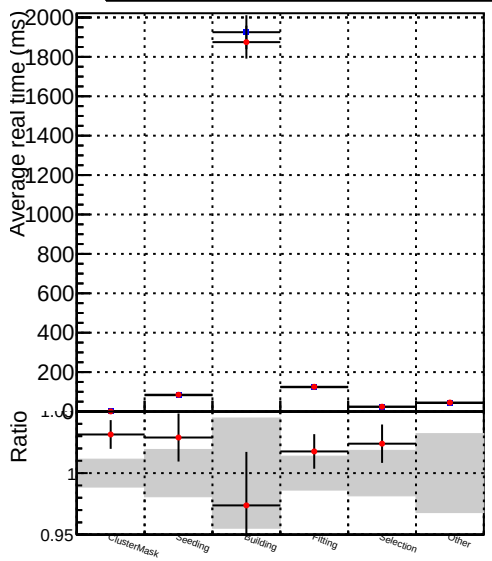
DQM_V0001_R000000001_Global_mkFit_baseline DQM_V0001_R000000001_Global_mkFit_BASELINE-2
