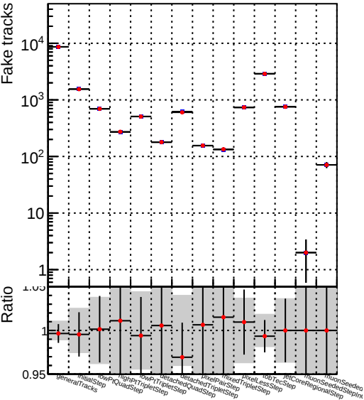
Number ● DQM_V0001_R000000001_Global_mkFit_BASELINE-2
