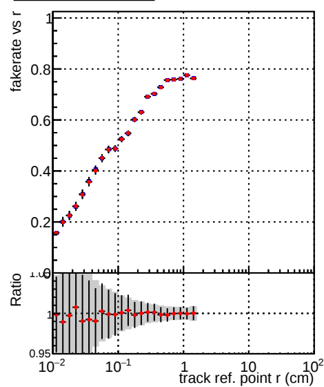
—●— DQM_V0001_R000000001_Global_mkFit_baseline —●— DQM_V0001_R000000001_Global_mkFit_BASELINE-2
