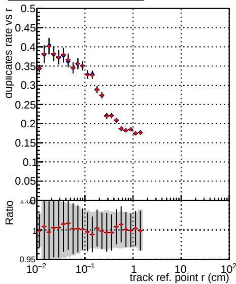
—●— DQM_V0001_R000000001_Global_mkFit_baseline —●— DQM_V0001_R000000001_Global_mkFit_BASELINE-2
