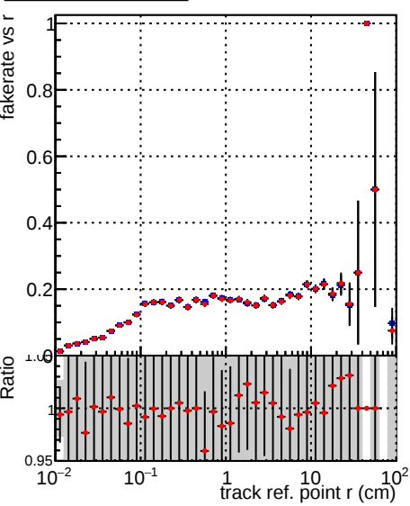
—•— DQM_V0001_R000000001_Global_mkFit_baseline —•— DQM_V0001_R000000001_Global_mkFit_BASELINE-2
