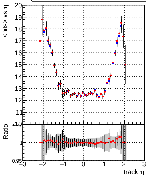
mean hits — DQM_V0001_R000000001_Global_mkFit_baseline — DQM_V0001_R000000001_Global_mkFit_BASELINE-2
