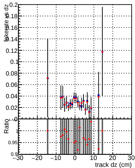
Fake rate vs dz DQM V0001_R000000001 Global mkFit baseline DQM V0001_R000000001 Global mkFit BASELINE-2
