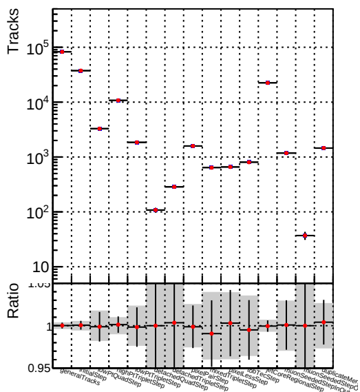
DQM_V0001_R000000001_Global_mkFit_baseline
