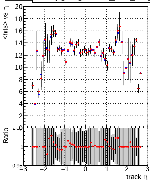
— DQM_V0001_R000000001_Global_mkFit_baseline — DQM_V0001_R000000001_Global_mkFit_BASELINE-2
