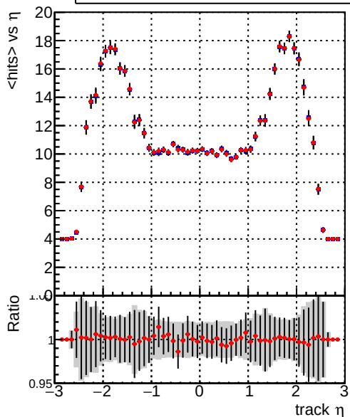
mean hits > vs \eta DQM_V0001_R000000001_Global_mkFit_BASELINE-2
