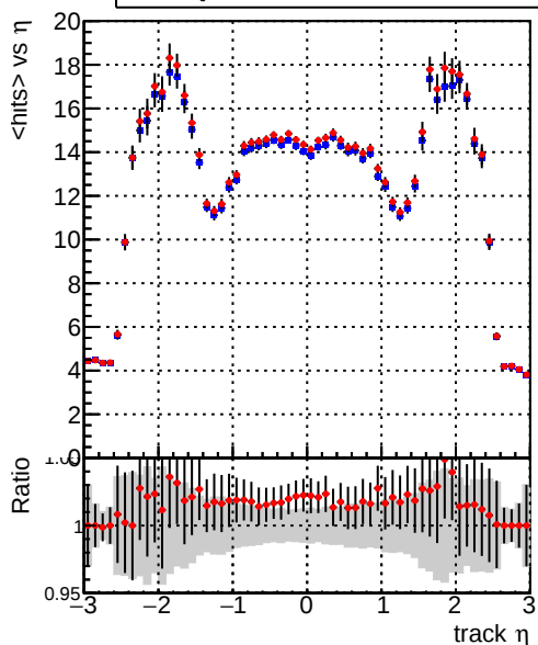
— DQM_V0001_R000000001_Global_mkFit_baseline — DQM_V0001_R000000001_Global_mkFit_BASELINE-2
