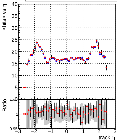
mean hit — DQM_V0001_R000000001_Global_mkFit_baseline — DQM_V0001_R000000001_Global_mkFit_BASELINE-2
