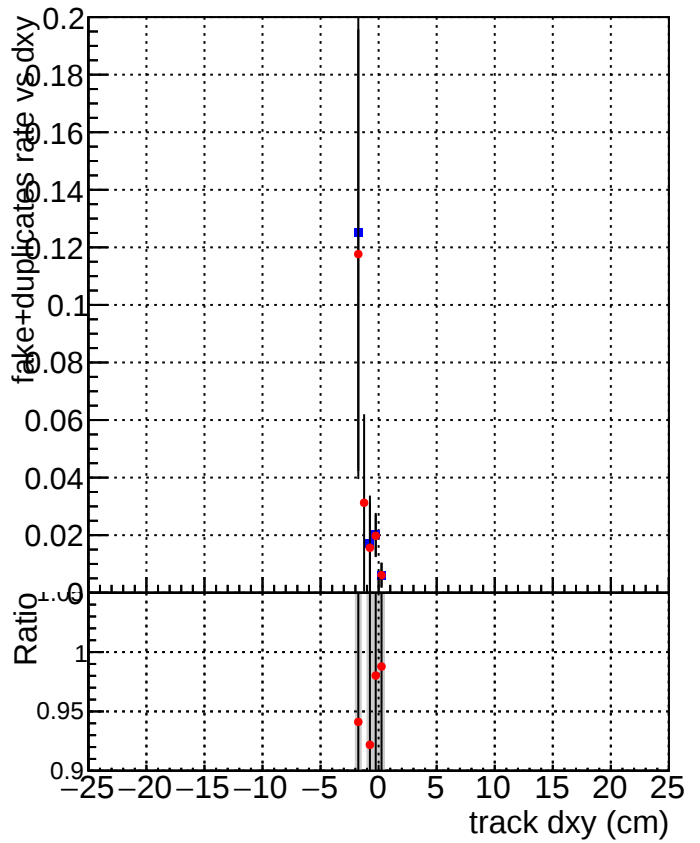
DQM_V0001_R000000001_Global_mkFit_baseline DQM_V0001_R000000001_Global_mkFit_BASELINE-2
