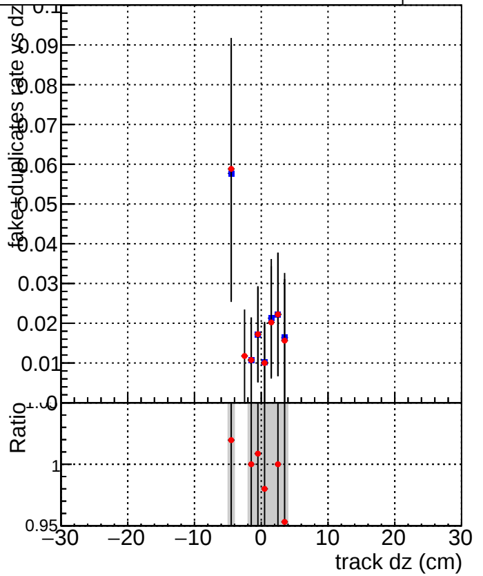
DQM_V0001_R000000001_Global_mkFit_baseline DQM_V0001_R000000001_Global_mkFit_BASELINE-2
