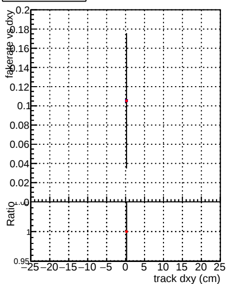
—•— DQM_V0001_R0000000001 Global mkFit baseline —•— DQM_V0001_R0000000001 Global mkFit BASELINE-2
