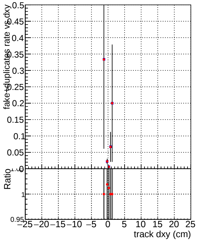
DQM_V0001_R0000000001_Global_mkFit_baseline DQM_V0001_R0000000001_Global_mkFit_BASELINE-2
