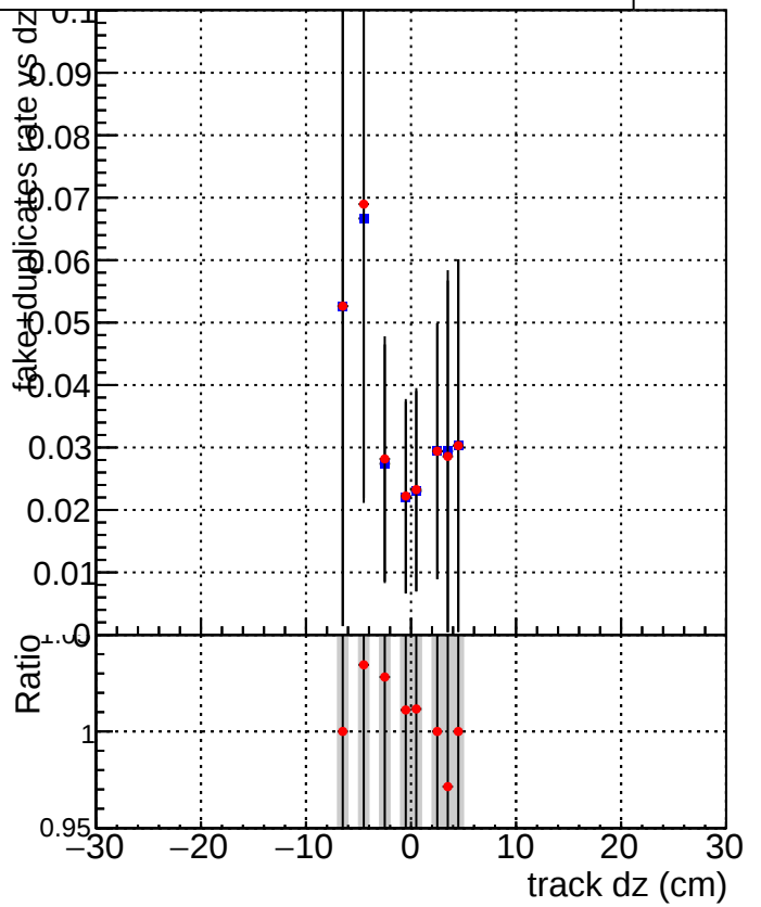
DQM_V0001_R0000000001_Global_mkFit_baseline DQM_V0001_R0000000001_Global_mkFit_BASELINE-2
