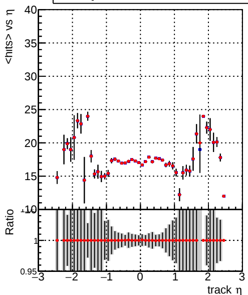
mean hit — DQM_V0001_R000000001_Global_mkFit_baseline — DQM_V0001_R000000001_Global_mkFit_BASELINE-2
