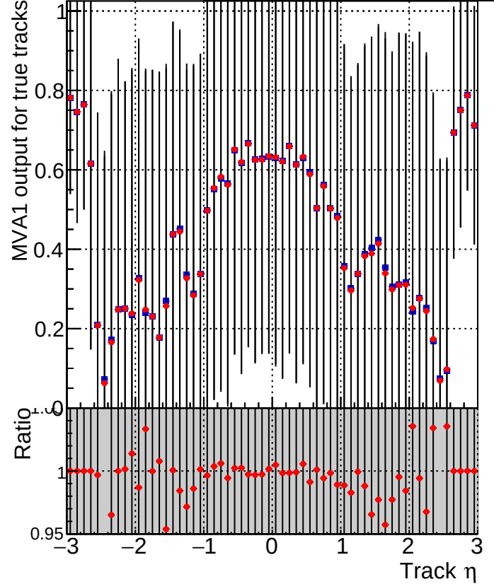
MVA1 of associated tracks (recoToSim) vs. track \eta Legend: ■ DQM_V0001_R000000001_Global_mkFit_baseline ■ DQM_V0001_R000000001_Global_mkFit_BASELINE-2
