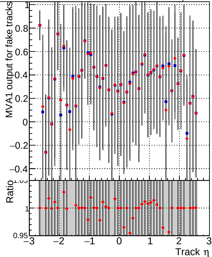
MVA1 of associated tracks (recoToSim) vs. track \eta ■ DQM_V0001_R000000001_Global_mkFit_baseline ● DQM_V0001_R000000001_Global_mkFit_BASELINE-2
