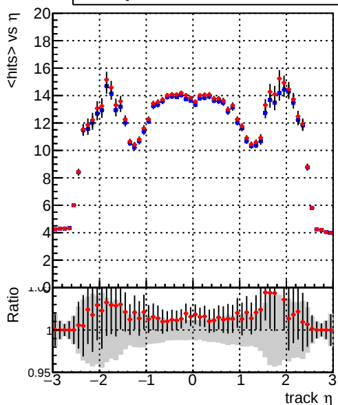
mean hits vs \eta — DQM_V0001_R000000001_Global_mkFit_baseline — DQM_V0001_R000000001_Global_mkFit_BASELINE-2
