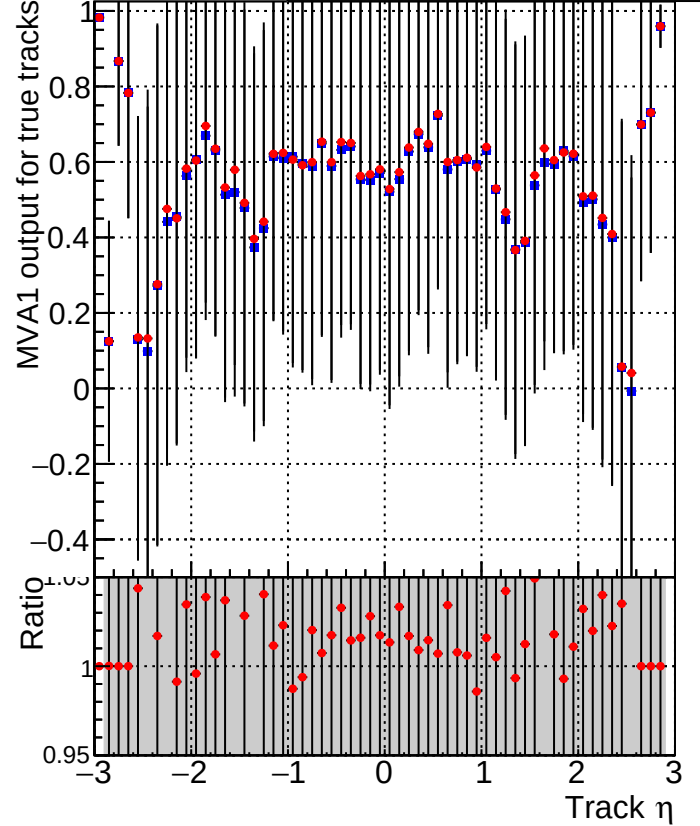
MVA1 of associated tracks (recoToSim) vs. track \eta Legend: Blue square: DQM_V0001_R000000001_Global_mkFit_baseline Red circle: DQM_V0001_R000000001_Global_mkFit_BASELINE-2
