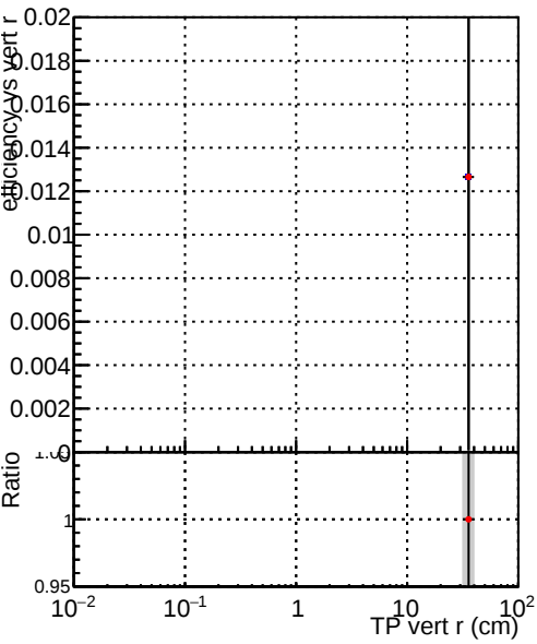
Efficiency vs vertpos Legend: DQM_V0001_R000000001_Global_mkFit_baseline DQM_V0001_R000000001_Global_mkFit_BASELINE-2
