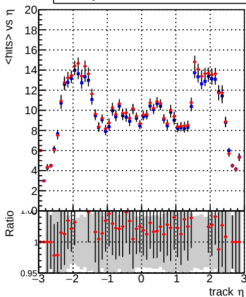
mean hits vs \eta Legend: DQM_V0001_R000000001_Global_mkFit_baseline (blue line), DQM_V0001_R000000001_Global_mkFit_BASELINE-2 (red line)
