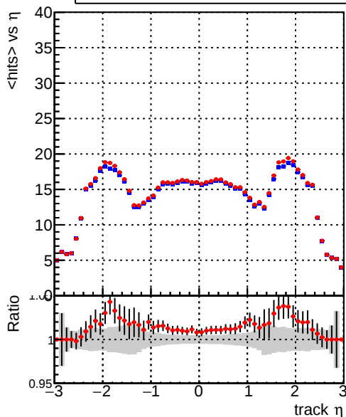
mean hit — DQM_V0001_R000000001_Global_mkFit_baseline — DQM_V0001_R000000001_Global_mkFit_BASELINE-2
