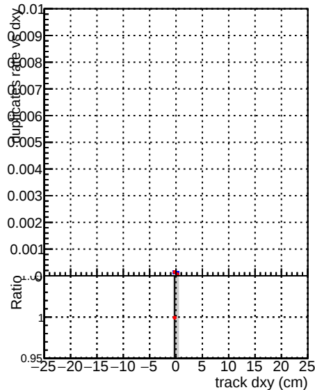
—●— DQM_V0001_R0000000001_Global_mkFit_baseline —●— DQM_V0001_R0000000001_Global_mkFit_BASELINE-2
