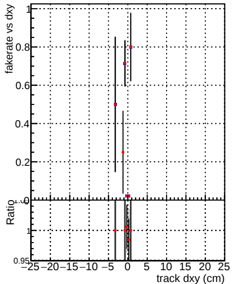
—●— DQM_V0001_R0000000001_Global_mkFit_baseline —●— DQM_V0001_R0000000001_Global_mkFit_BASELINE-2
