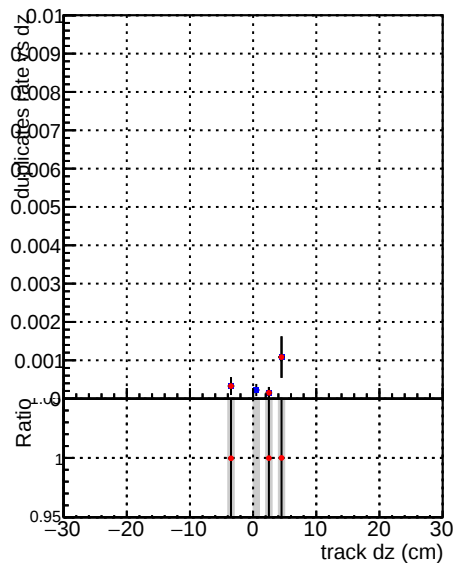
—●— DQM_V0001_R0000000001_Global_mkFit_baseline —●— DQM_V0001_R0000000001_Global_mkFit_BASELINE-2
