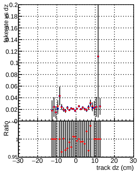
—●— DQM_V0001_R0000000001_Global_mkFit_baseline —●— DQM_V0001_R0000000001_Global_mkFit_BASELINE-2
