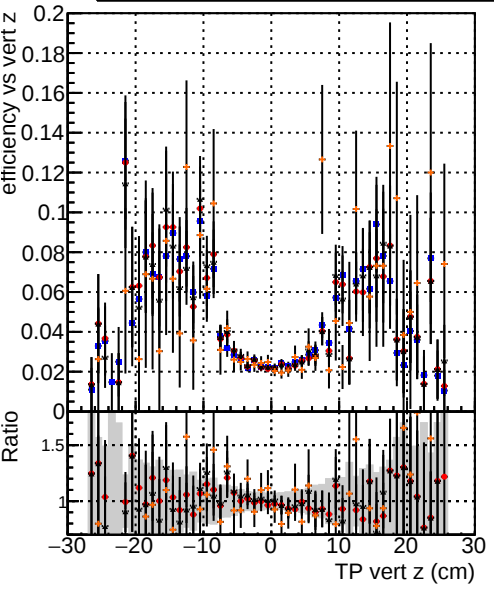
Efficiency vs vertpos —●— DQM_V0001_R000000001 Global_mkFit_baseline —●— DQM_V0001_R000000001 Global_mkFit_var —●— DQM_V0001_R000000001 Global_mkFit_jcoreNoClean —●— DQM_V0001_R000000001 Global_mkFit_jcore50maxCand-33DUPremoval
