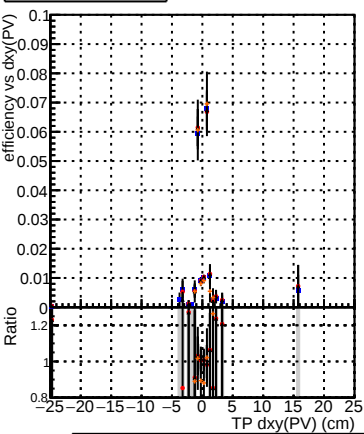
Efficiency vs Dxy(PV) Legend: DQM_V0001_R0000000001_Global_mkFit_baseline DQM_V0001_R0000000001_Global_mkFit_var DQM_V0001_R0000000001_Global_mkFit_jcoreNoClean DQM_V0001_R0000000001_Global_mkFit_jcore50maxCand-33DUPremoval
