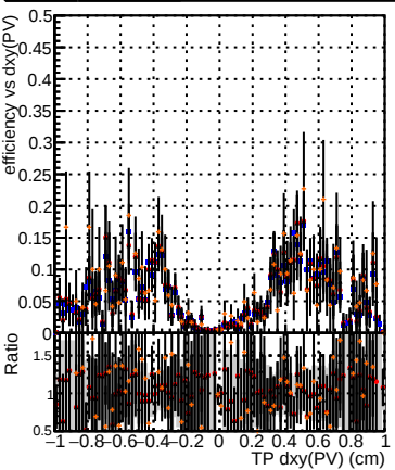
Efficiency vs Dxy(PV) Legend: DQM_V0001_R0000000001_Global_mkFit_baseline DQM_V0001_R0000000001_Global_mkFit_var DQM_V0001_R0000000001_Global_mkFit_jcoreNoClean DQM_V0001_R0000000001_Global_mkFit_jcore50maxCand-33DUPremoval
