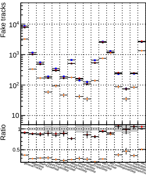
Number — DQM_V0001_R0000000001 Global mkFit jcoreNoClean + DQM_V0001_R0000000001 Global mkFit jcore50maxCand-33DUPremoval
