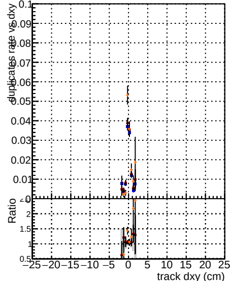
al=mkFit=coreNoClean al=mkFit=core50maxCand-33DUPremoval
