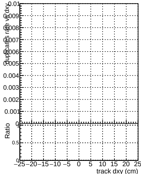
al=mkFit=coreNoClean al=mkFit=core50maxCand-33DUPremoval
