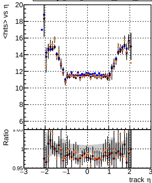
mean hits vs \eta Legend: DQM_V0001_R000000001_Global_mkFit_baseline (blue line), DQM_V0001_R000000001_Global_mkFit_var (red line), DQM_V0001_R000000001_Global_mkFit_coreNoClean (black line), DQM_V0001_R000000001_Global_mkFit_core50maxCand-33DUPremoval (orange line)
