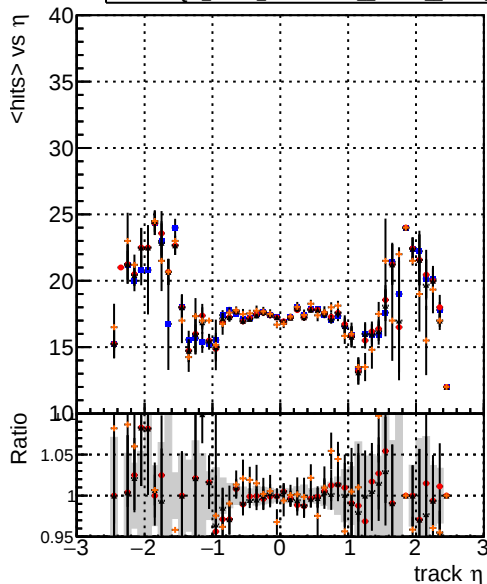
mean hits vs \eta Legend: DQM_V0001_R000000001_Global_mkFit_baseline (blue line), DQM_V0001_R000000001_Global_mkFit_var (red line), DQM_V0001_R000000001_Global_mkFit_jcoreNoClean (black line), DQM_V0001_R000000001_Global_mkFit_icore50maxCand-33DUPremoval (orange line)
