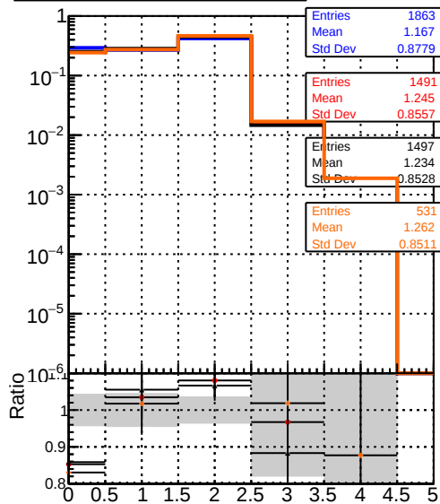
Legend for mean hits vs \eta : DQM_V0001_R000000001_Global_mkFit_baseline DQM_V0001_R000000001_Global_mkFit_var DQM_V0001_R000000001_Global_mkFit_coreNoClean DQM_V0001_R000000001_Global_mkFit_core50maxCand-33DUPremoval
