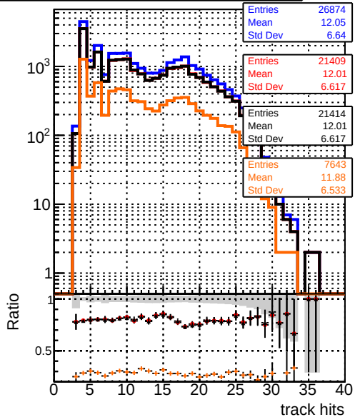
mean hits Legend: DQM_V0001_R0000000001_Global_mkFit_baseline DQM_V0001_R0000000001_Global_mkFit_var DQM_V0001_R0000000001_Global_mkFit_coreNoClean DQM_V0001_R0000000001_Global_mkFit_core50maxCand-33DUPremoval
