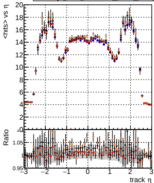
mean hit DQM_V0001_R0000000001 Global mkFit baseline DQM_V0001_R0000000001 Global mkFit var DQM_V0001_R0000000001 Global mkFit jcoreNoClean DQM_V0001_R0000000001 Global mkFit jcore50maxCand-33DUPremoval
