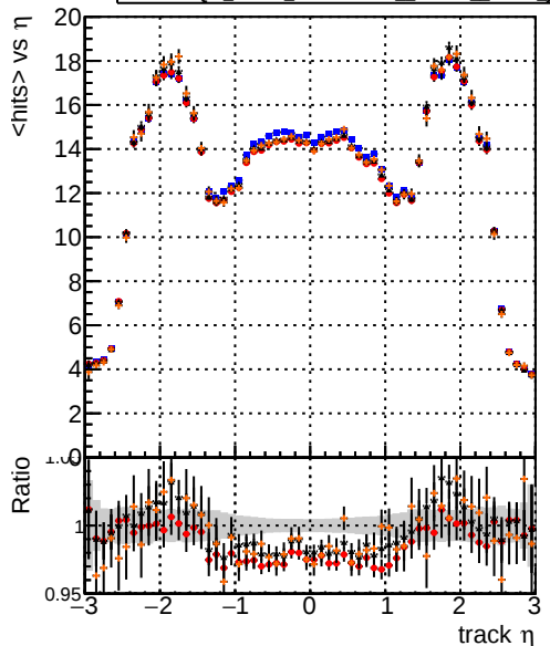
mean hits vs \eta Legend: Global mkFit baseline (blue line) Global mkFit var (red line) Global mkFit jcoreNoClean (black line) Global mkFit jcore50maxCand-33DUPremoval (orange line)
