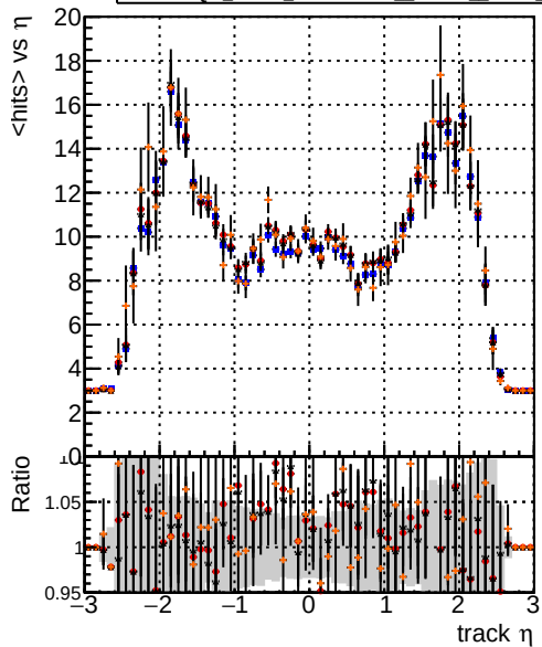
mean hits vs \eta — DQM_V0001_R000000001_Global_mkFit_baseline — DQM_V0001_R000000001_Global_mkFit_var — DQM_V0001_R000000001_Global_mkFit_coreNoClean — DQM_V0001_R000000001_Global_mkFit_core50maxCand-33DUPremoval
