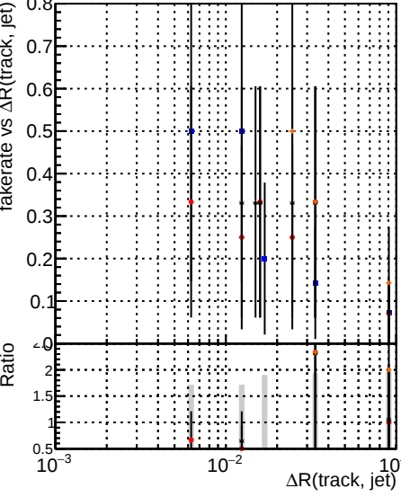
Fake rate vs \Delta R(\text{track, jet}) DQM V00001 R000000000001 Global mkFit baseline Global mkFit var Global mkFit coreNoClean Global mkFit core50maxCand-33DUPremoval
