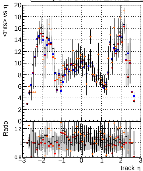
mean hits vs \eta Legend: DQM_V0001_R0000000001_Global_mkFit_baseline DQM_V0001_R0000000001_Global_mkFit_var DQM_V0001_R0000000001_Global_mkFit_coreNoClean DQM_V0001_R0000000001_Global_mkFit_core50maxCand-33DUPremoval
