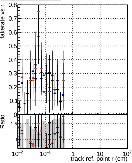
Fake rate vs v Global mkFit baseline Global mkFit var Global mkFit coreNoClean Global mkFit core50maxCand-33DUPremoval
