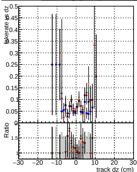
Fake rate vs dz Legend: BSM V0001 (blue), BSM V0001 R0000000001 (orange), Global fit baseline (grey), Global fit var (black), Global fit (red), Global fit Clean (green), Global fit core30maxCand-33DUPremoval (purple), Global fit (dark blue).
