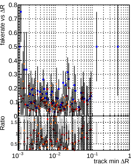
Fake rate vs \Delta R(\text{track, jet}) DQM V00001 R00000000001 Global mkFit baseline Global mkFit var Global mkFit coreNoClean Global mkFit core50maxCand-33DUPremoval
