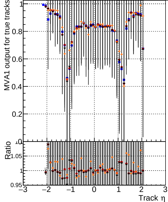
MVA1 of associated tracks (recoToSim) vs. track \eta ■ DQM_V0001_R0000000001 Global mkFit_baseline ● DQM_V0001_R0000000001 Global mkFit_var ▲ DQM_V0001_R0000000001 Global mkFit_coreNoClean ✕ DQM_V0001_R0000000001 Global mkFit_core50maxCand-33DUPremoval
