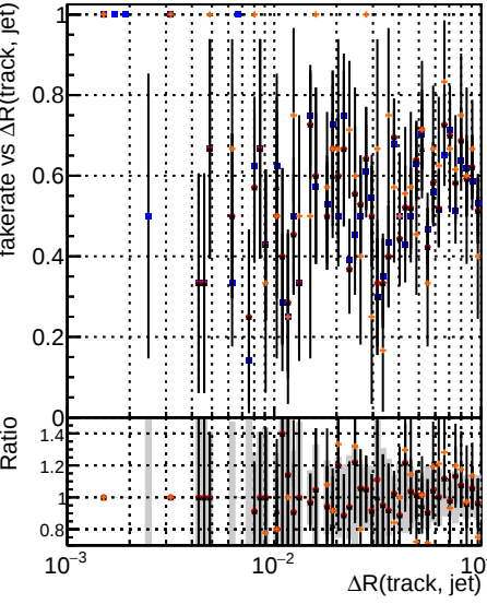
Fake rate vs \Delta R (track, jet) Legend: Global mkFit baseline (black line), Global mkFit var (blue line), Global mkFit core50maxCand-33DUPremoval (orange line), Global mkFit core50maxCand-33DUPremoval (red line). Global mkFit baseline Global mkFit var Global mkFit core50maxCand-33DUPremoval Global mkFit core50maxCand-33DUPremoval
