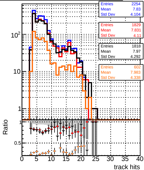
mean hit DQM_V0001_R000000001_Global_mkFit_baseline DQM_V0001_R000000001_Global_mkFit_var DQM_V0001_R000000001_Global_mkFit_coreNoClean DQM_V0001_R000000001_Global_mkFit_core50maxCand-33DUPremoval
