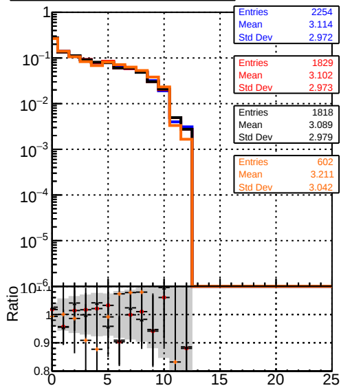
mean hit DQM_V0001_R000000001_Global_mkFit_baseline DQM_V0001_R000000001_Global_mkFit_var DQM_V0001_R000000001_Global_mkFit_coreNoClean DQM_V0001_R000000001_Global_mkFit_core50maxCand-33DUPremoval
