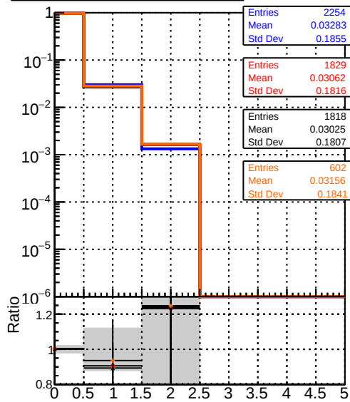
mean hit DQM_V0001_R000000001_Global_mkFit_baseline DQM_V0001_R000000001_Global_mkFit_var DQM_V0001_R000000001_Global_mkFit_coreNoClean DQM_V0001_R000000001_Global_mkFit_core50maxCand-33DUPremoval
