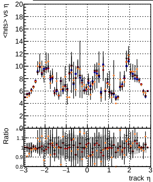
mean hit DQM_V0001_R000000001_Global_mkFit_baseline DQM_V0001_R000000001_Global_mkFit_var DQM_V0001_R000000001_Global_mkFit_coreNoClean DQM_V0001_R000000001_Global_mkFit_core50maxCand-33DUPremoval
