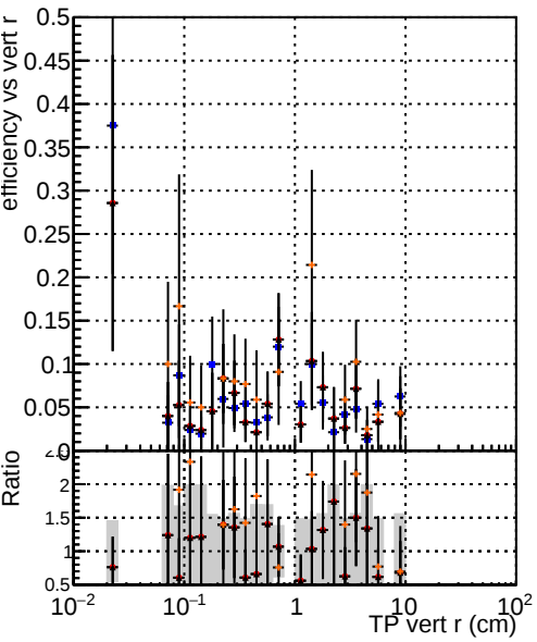
Efficiency vs TP vert r (cm) Global_mkFit_baseline Global_mkFit_var Global_mkFit_jcoreNoClean Global_mkFit_jcore50maxCand-33DUPremoval
