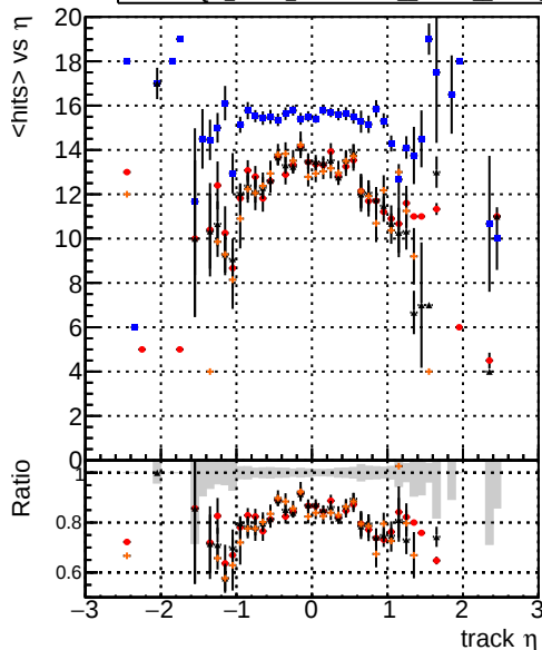
mean hits vs \eta Legend: Global mkFit baseline (blue line) Global mkFit var (red line) Global mkFit jcoreNoClean (black line) Global mkFit jcore50maxCand-33DUPremoval (orange line)
