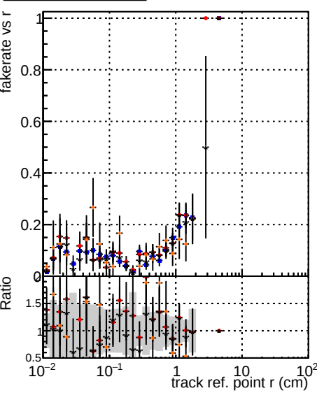
Fake rate vs verpos Global mkFit baseline Global mkFit var Global mkFit coreNoClean Global mkFit core50maxCand-33DUPremoval BQM V00001 R00000000001
