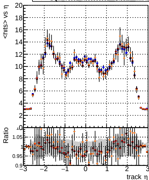
mean hits vs \eta Legend: DQM_V0001_R0000000001 Global mkFit baseline (blue), DQM_V0001_R0000000001 Global mkFit var (red), DQM_V0001_R0000000001 Global mkFit jcoreNoClean (black), DQM_V0001_R0000000001 Global mkFit jcore50maxCand-33DUPremoval (orange)
