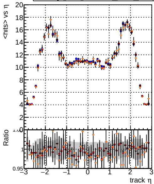
mean hits vs \eta Legend: DQM_V0001_R000000001_Global_mkFit_baseline, DQM_V0001_R000000001_Global_mkFit_var, DQM_V0001_R000000001_Global_mkFit_coreNoClean, DQM_V0001_R000000001_Global_mkFit_core50maxCand-33DUPremoval
