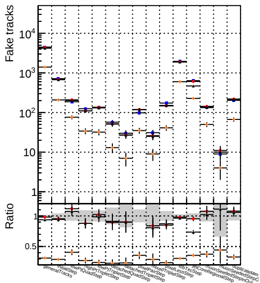
Number DQM_V0001_R0000000001_Global_mkFit_baseline DQM_V0001_R0000000001_Global_mkFit_var DQM_V0001_R0000000001_Global_mkFit_jcoreNoClean DQM_V0001_R0000000001_Global_mkFit_jcore50maxCand-24DUPremoval
