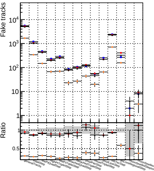
Number — DQM_V0001_R0000000001 Global mkFit jcoreNoClean + DQM_V0001_R0000000001 Global mkFit jcore50maxCand-24DUPremoval
